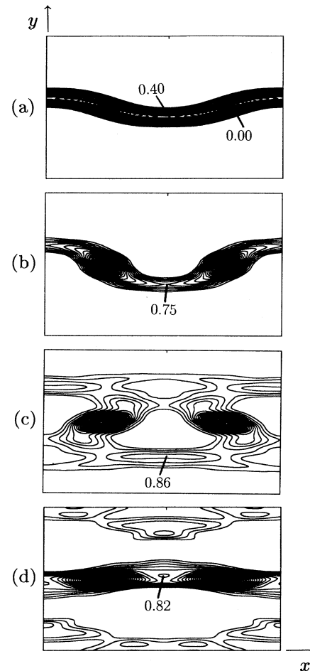
FIG. 7. Development of the transverse instability for the large-amplitude dark soliton at k = 1.0 , p = 0.4 [point C in Fig. 1(a)]: (a) t = 3 , (b) t = 6 , (c) t = 9 , and (d) t = 13 . Creation of pairs of optical vortex and antivortex solitons is observed.
